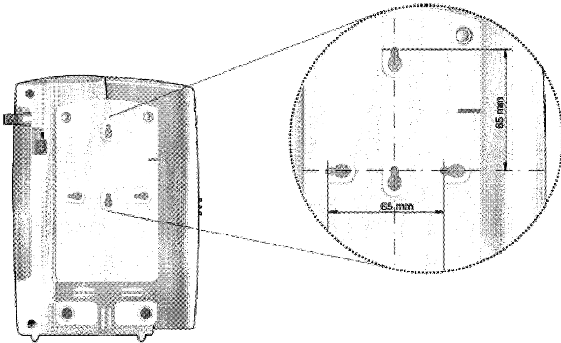
Mounting Template
